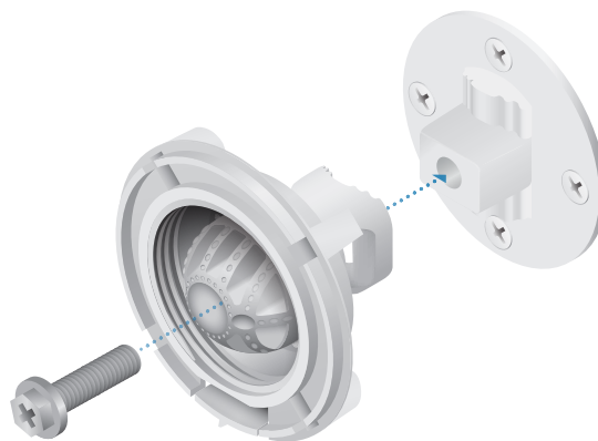
Mount Assembly
