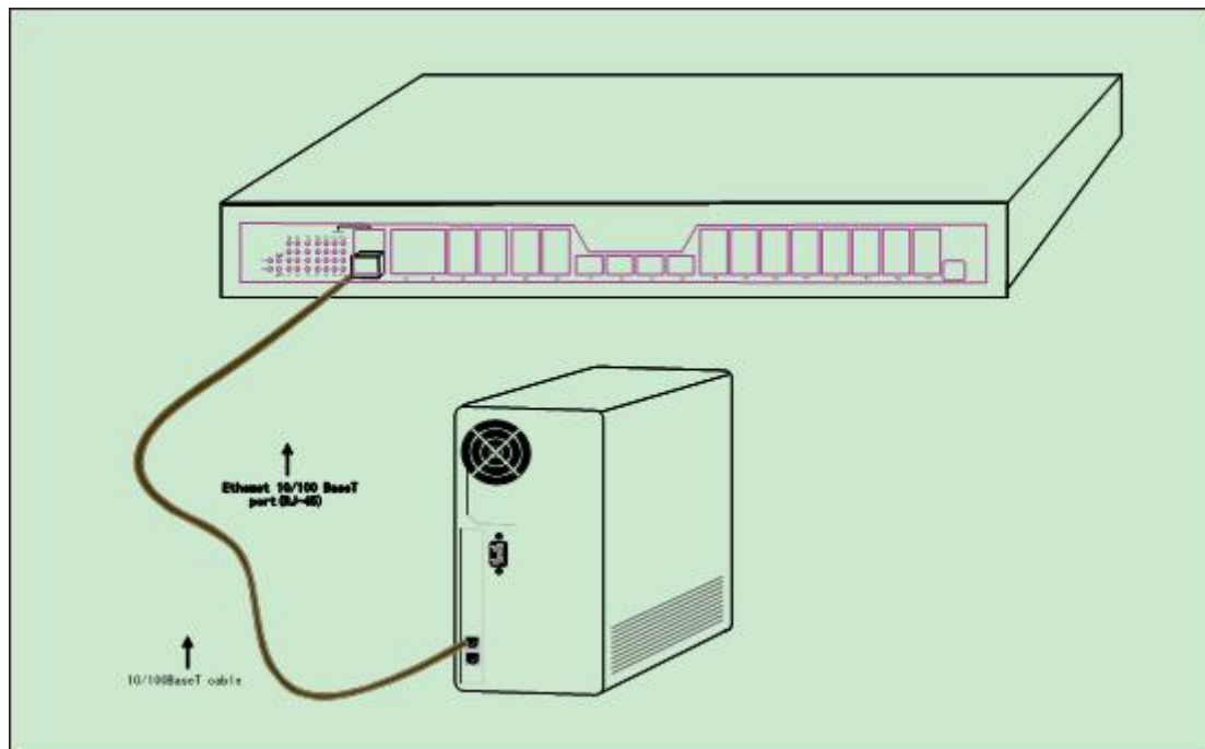
Figure 3-4 Connecting the console port of BDCOM GP3600-08 GPON and the computer
