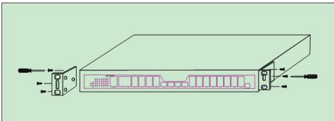
Figure 3-1 Fixing the machine box of BDCOM GP3600-08 GPON to the cabinet
