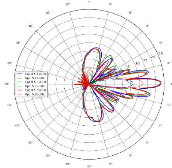
Azimuth Vertical
