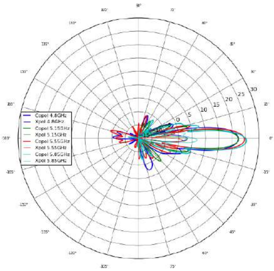
Azimuth Horizontal
