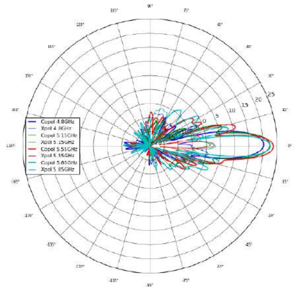
Elevation Vertical
