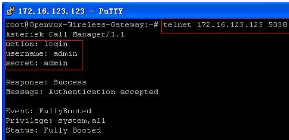
Figure 8-1-2 Putty Access
