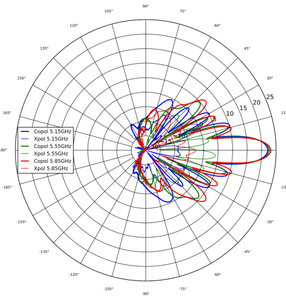
5 GHz Azimuth
