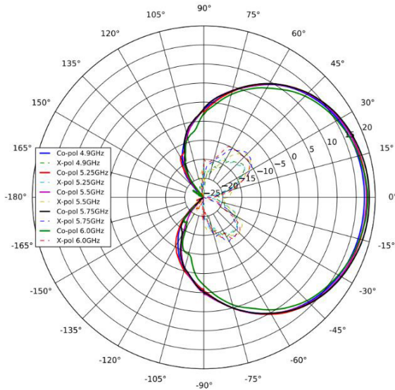
5 GHz Azimuth
