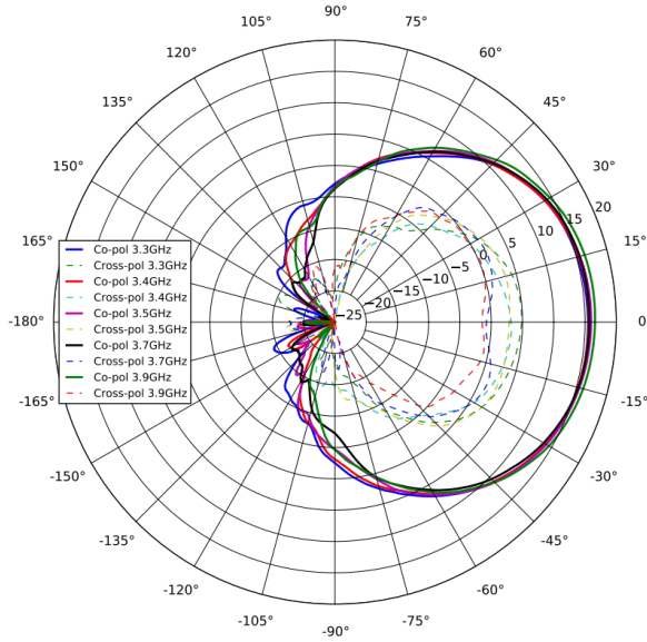
3 GHz Azimuth
