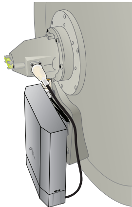
Connecting to a Dish Antenna
