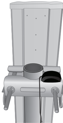
Recommended Placement of GPS Patch Antenna on a Sector Antenna
