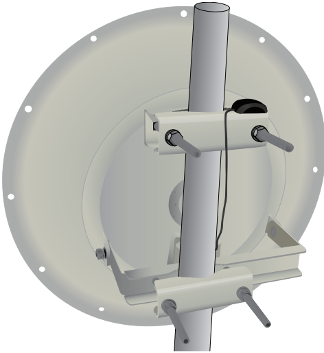
Recommended Placement of GPS Patch Antenna on a Dish Antenna
