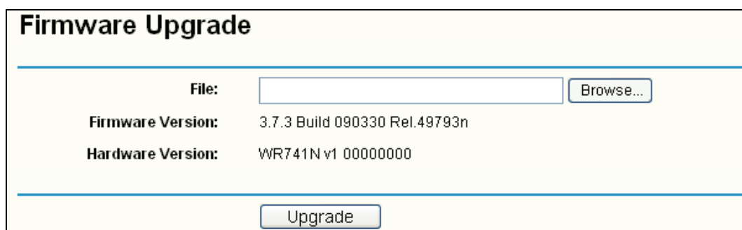
Figure 4-73 Firmware Upgrade
