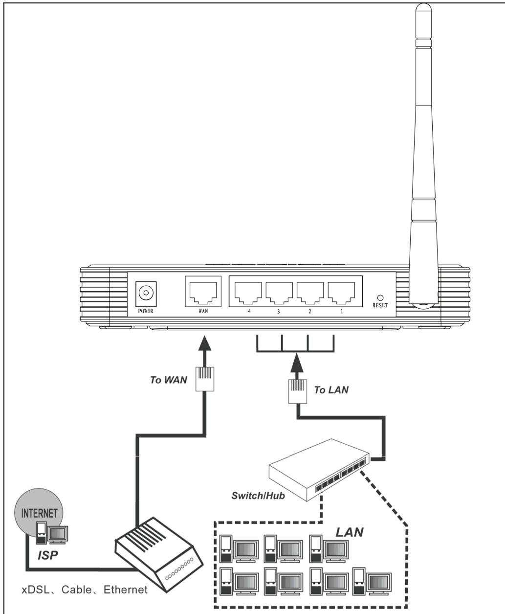
Figure 2-1 Hardware Installation of the TL-WR741ND 150Mbps Wireless Lite-N Router
