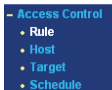
Figure 4-45 Access Control
