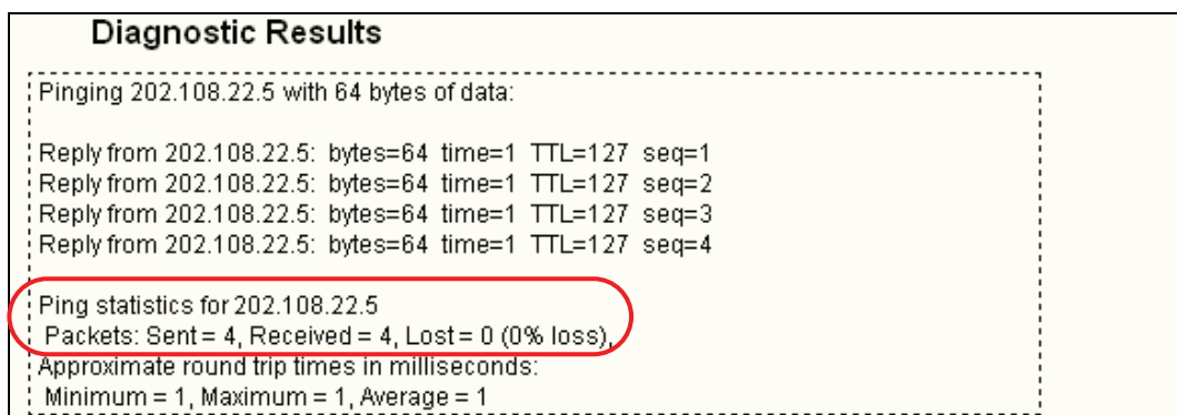
Figure 4-72 Diagnostic Results
