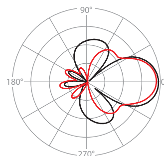
Elevation Pattern (H / V)
