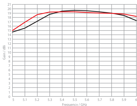
Gain (H / V)
