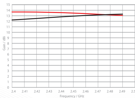
Gain (H / V)
